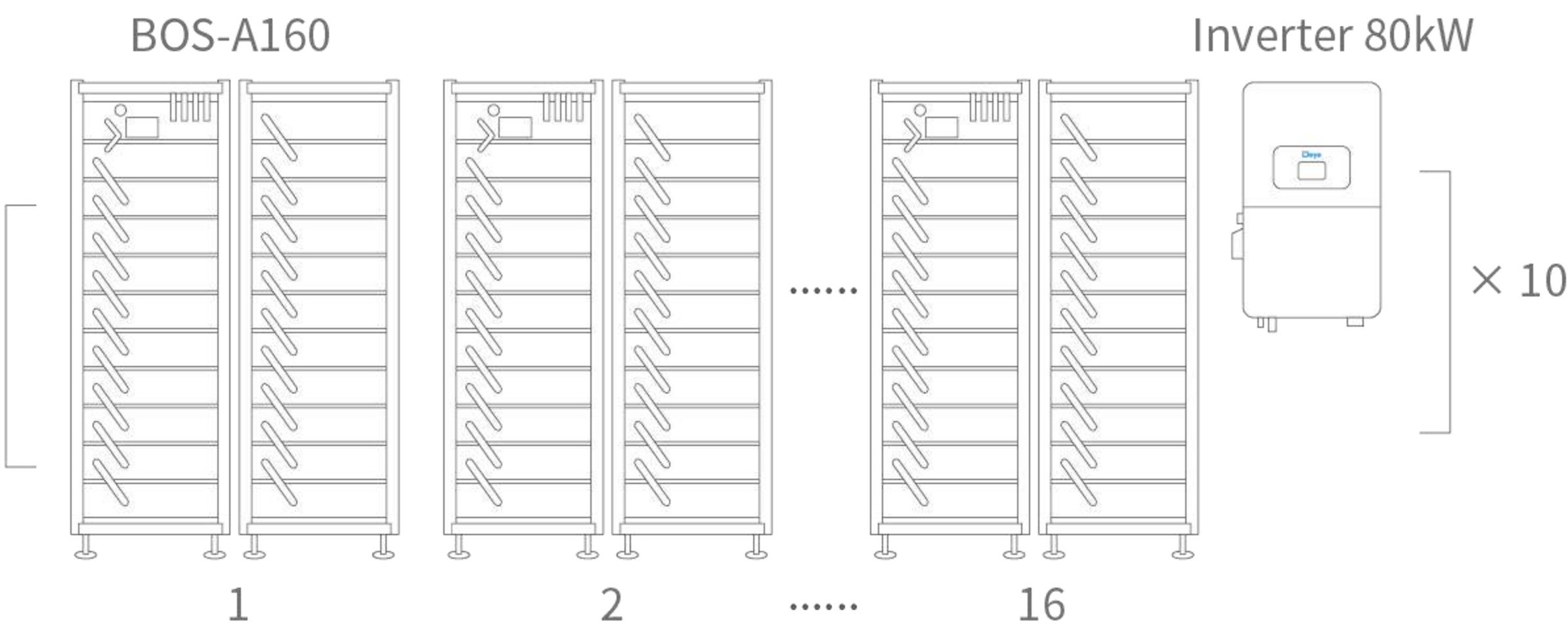
Maximum support for 10 inverters in AC parallel operation
